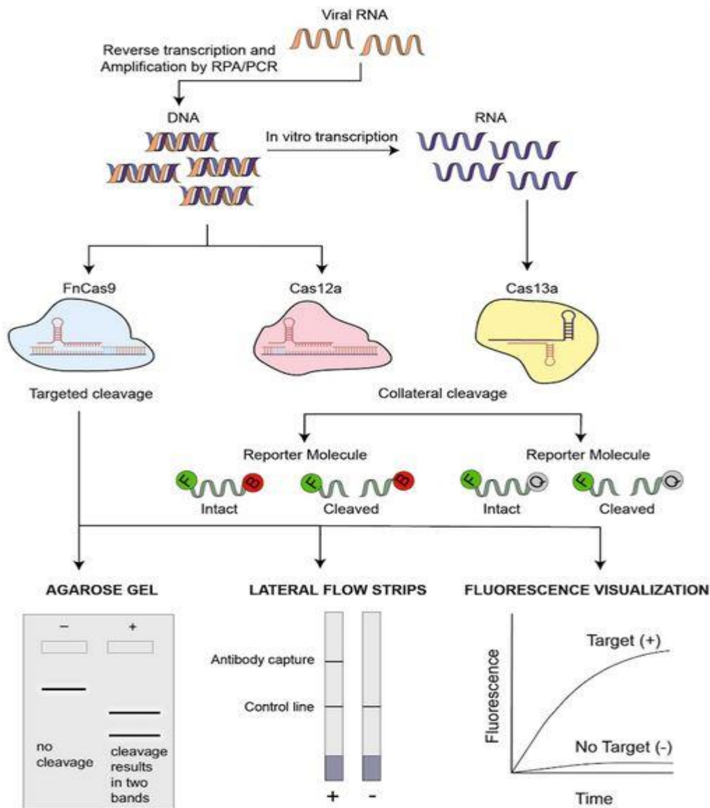
Fig. 1. An overview of the general schematic of CRISPR/Cas based COVID-19 testing methods [36].
